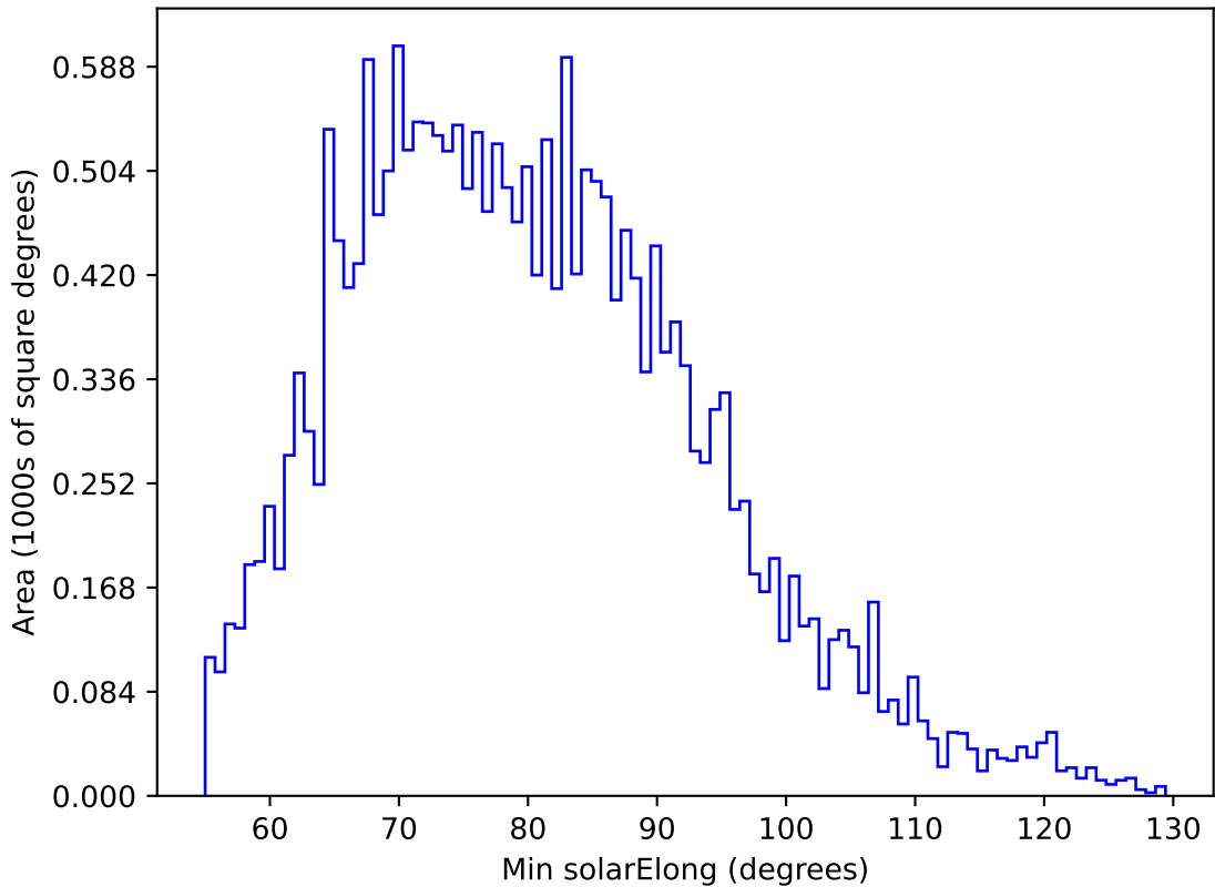
too_elab_heavy_r32_d2_gz_v3.4_10yrs All sky u band: Min solarElong
