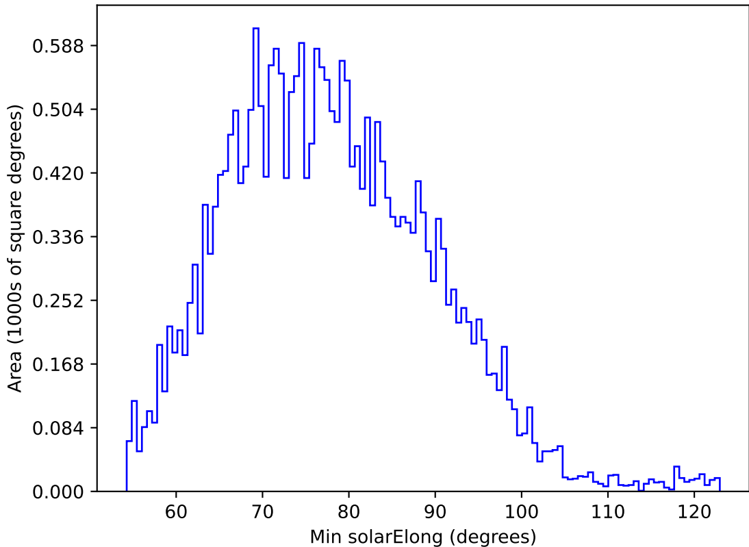
too_elab_heavy_r32_d2_gz_v3.4_10yrs All sky g band: Min solarElong
