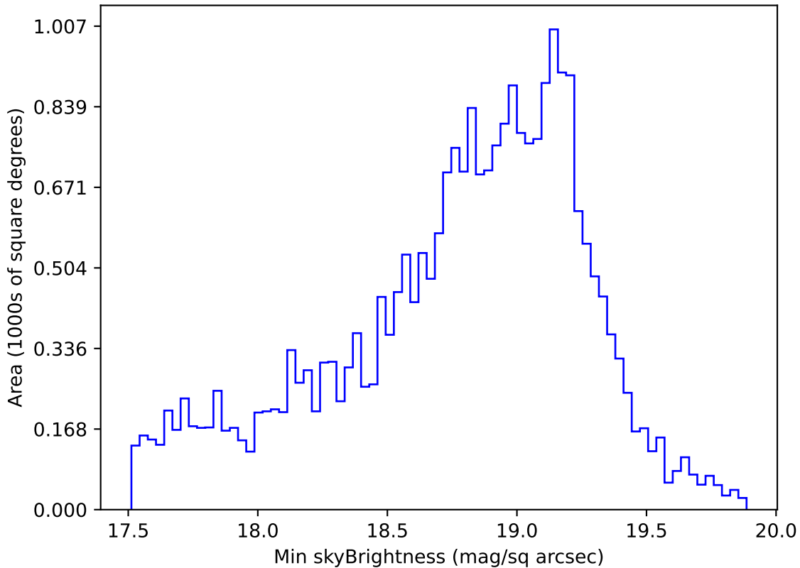
too_elab_heavy_r32_d2_gz_v3.4_10yrs Yr 1 i band: Min skyBrightness
