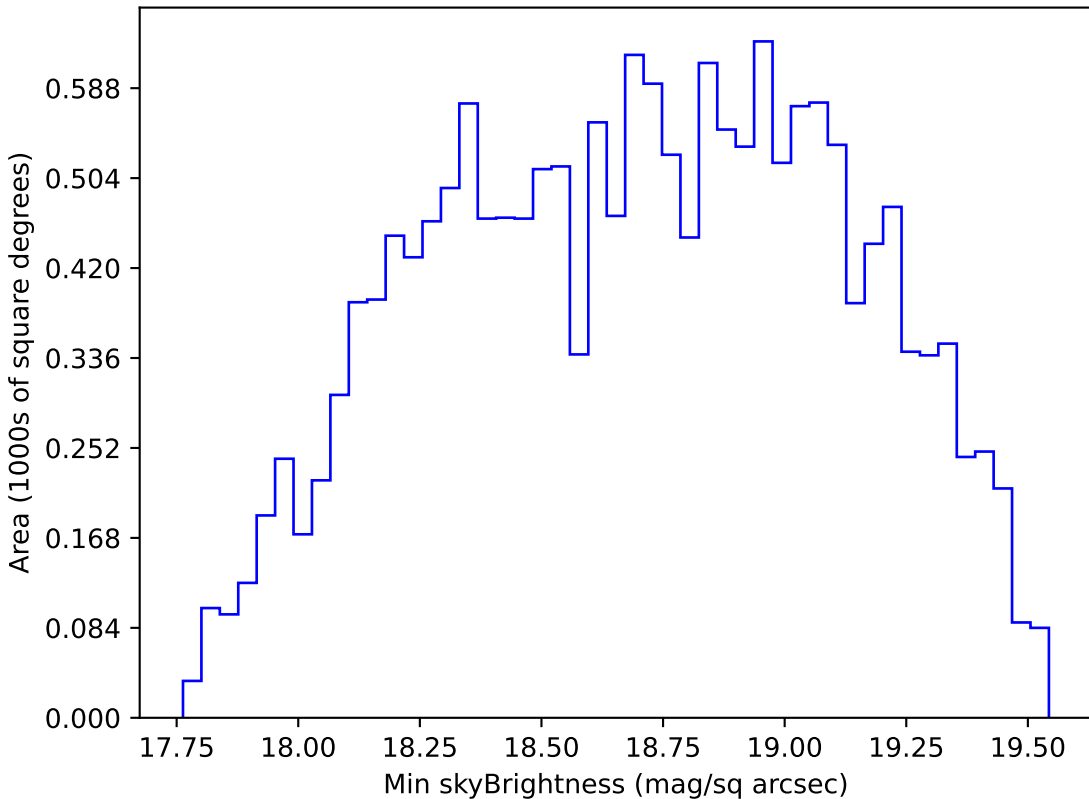
too_elab_heavy_r32_d2_gz_v3.4_10yrs WFD r band: Min skyBrightness
