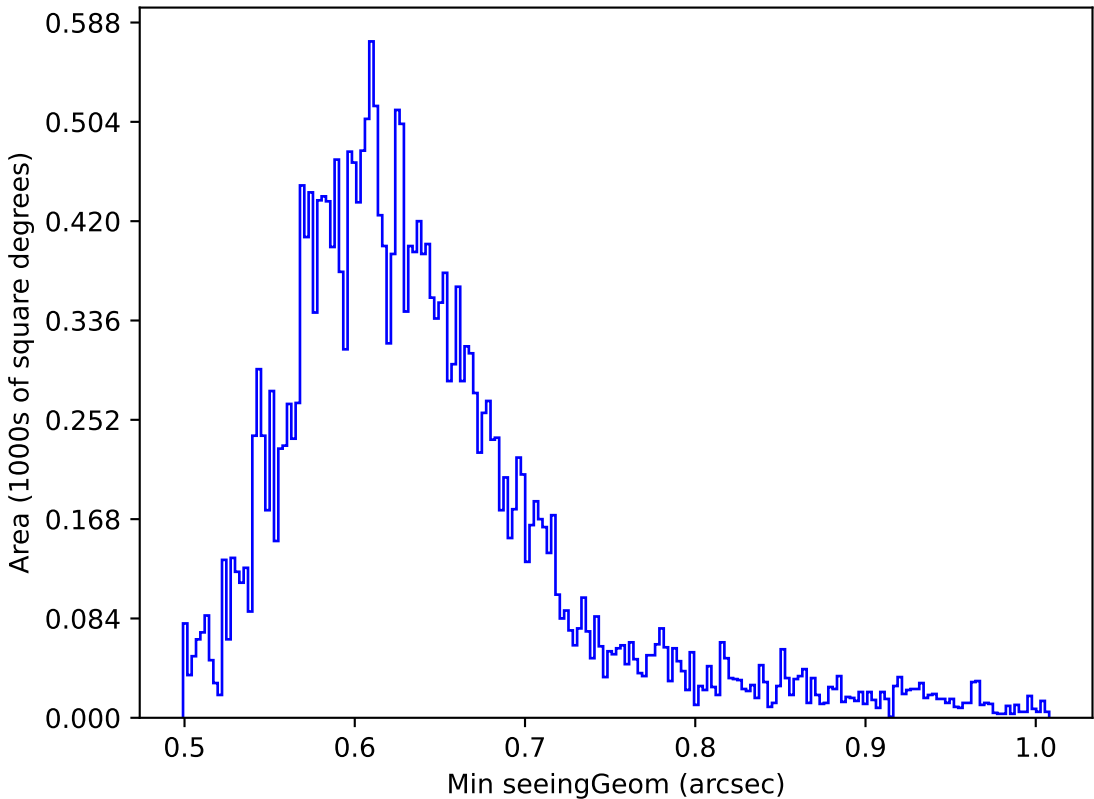
too_elab_heavy_r32_d2_gz_v3.4_10yrs Yr 1 z band: Min seeingGeom
