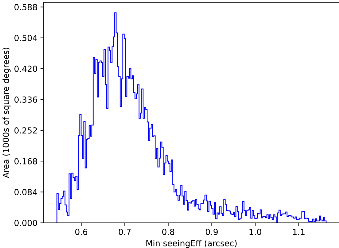
too_elab_heavy_r32_d2_gz_v3.4_10yrs Yr 1 z band: Min seeingEff
