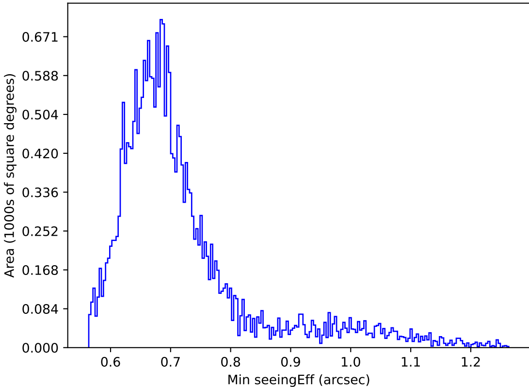
too_elab_heavy_r32_d2_gz_v3.4_10yrs Yr 1 r band: Min seeingEff
