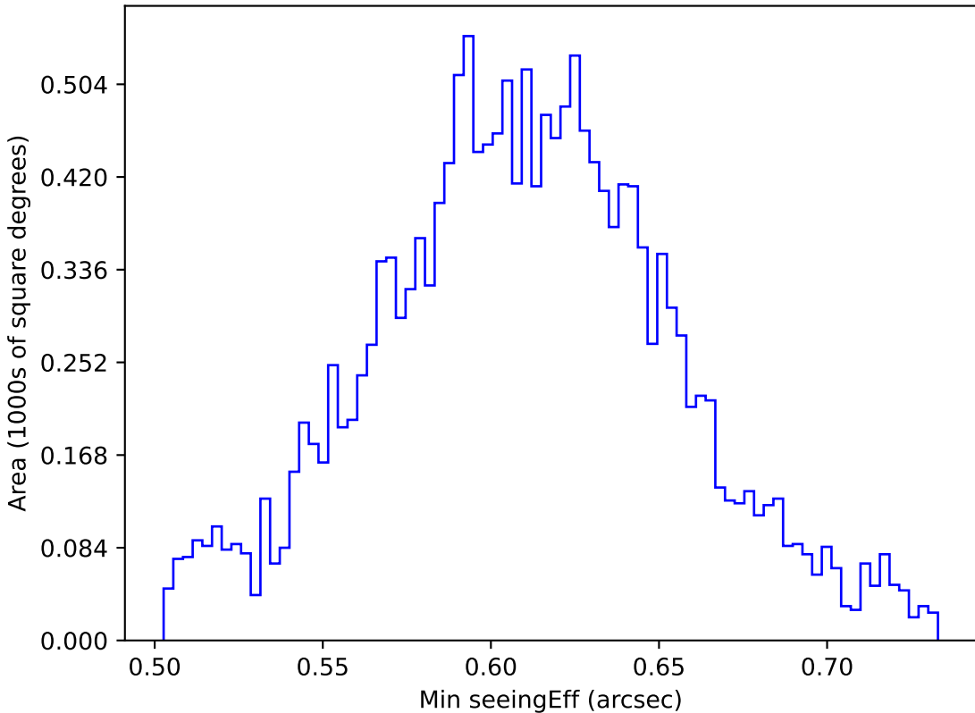
too_elab_heavy_r32_d2_gz_v3.4_10yrs WFD r band: Min seeingEff
