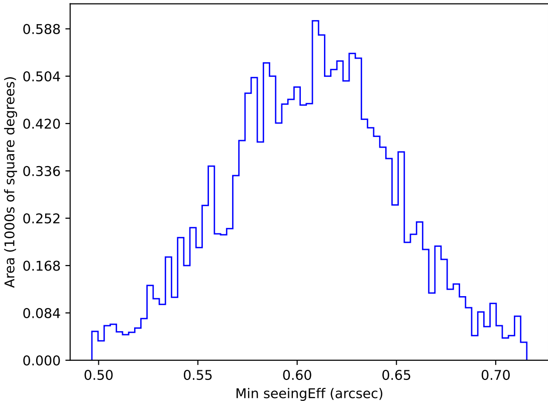
too_elab_heavy_r32_d2_gz_v3.4_10yrs WFD i band: Min seeingEff
