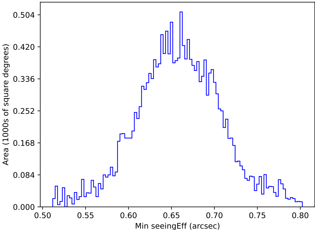
too_elab_heavy_r32_d2_gz_v3.4_10yrs WFD g band: Min seeingEff
