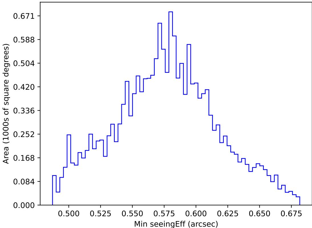
too_elab_heavy_r32_d2_gz_v3.4_10yrs WFD all bands: Min seeingEff
