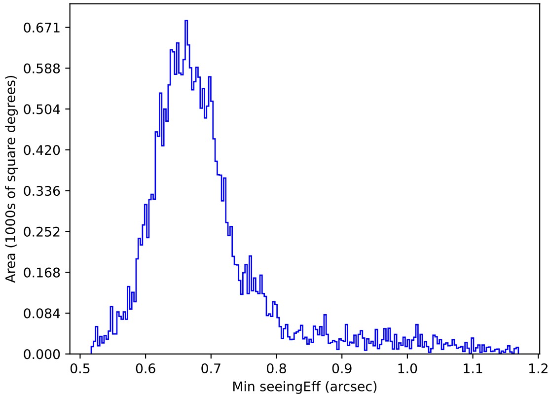
too_elab_heavy_r32_d2_gz_v3.4_10yrs All sky g band: Min seeingEff
