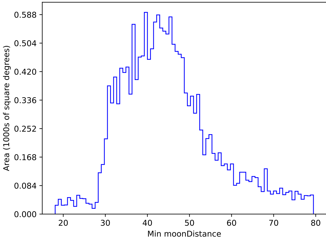
too_elab_heavy_r32_d2_gz_v3.4_10yrs WFD g band: Min moonDistance
