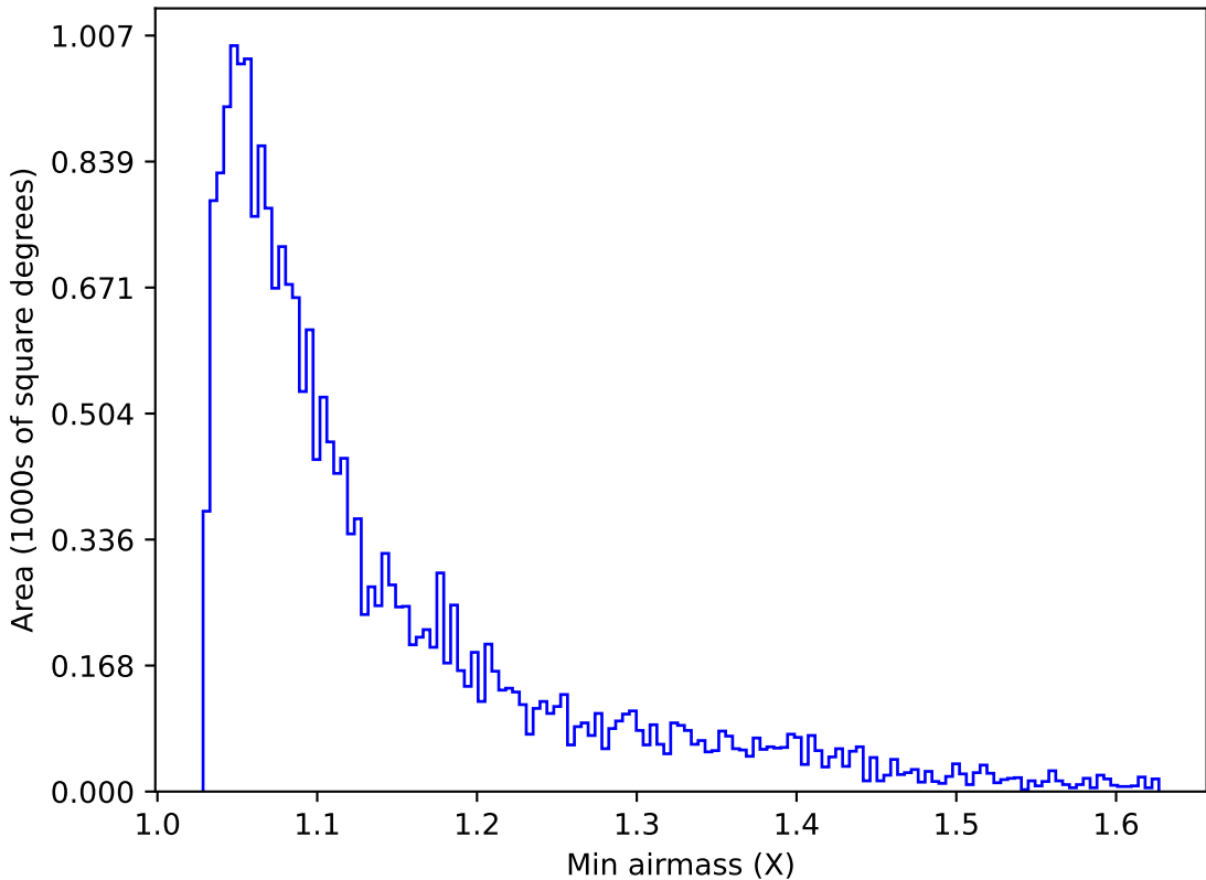
too_elab_heavy_r32_d2_gz_v3.4_10yrs Yr 1 u band: Min airmass
