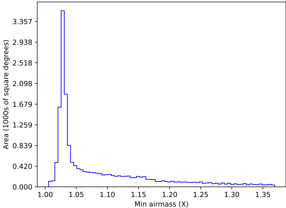
too_elab_heavy_r32_d2_gz_v3.4_10yrs WFD z band: Min airmass
