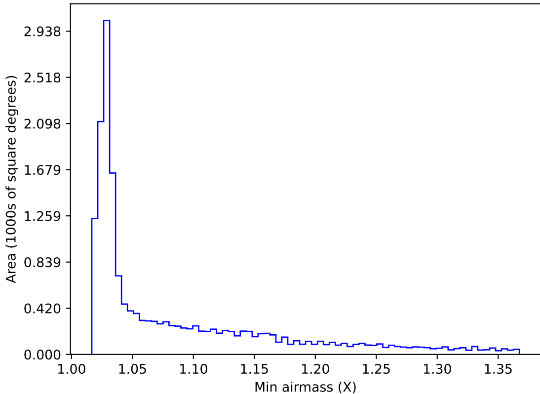
too_elab_heavy_r32_d2_gz_v3.4_10yrs WFD r band: Min airmass
