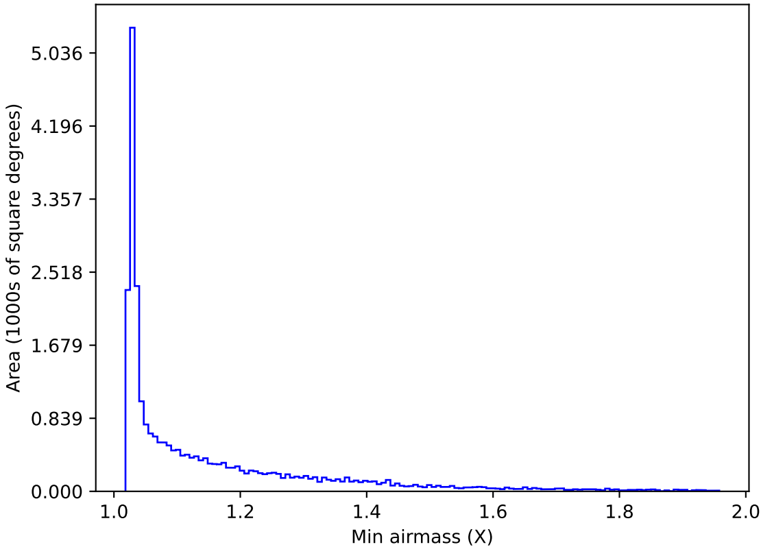
too_elab_heavy_r32_d2_gz_v3.4_10yrs All sky i band: Min airmass
