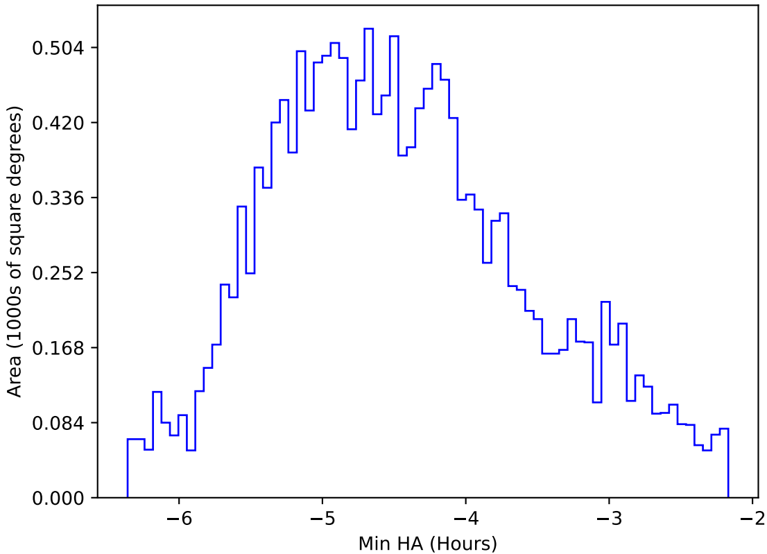
too_elab_heavy_r32_d2_gz_v3.4_10yrs WFD r band: Min HA
