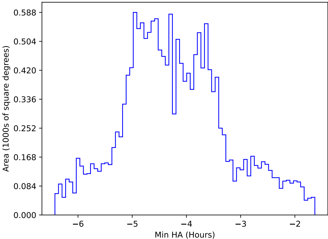
too_elab_heavy_r32_d2_gz_v3.4_10yrs WFD g band: Min HA
