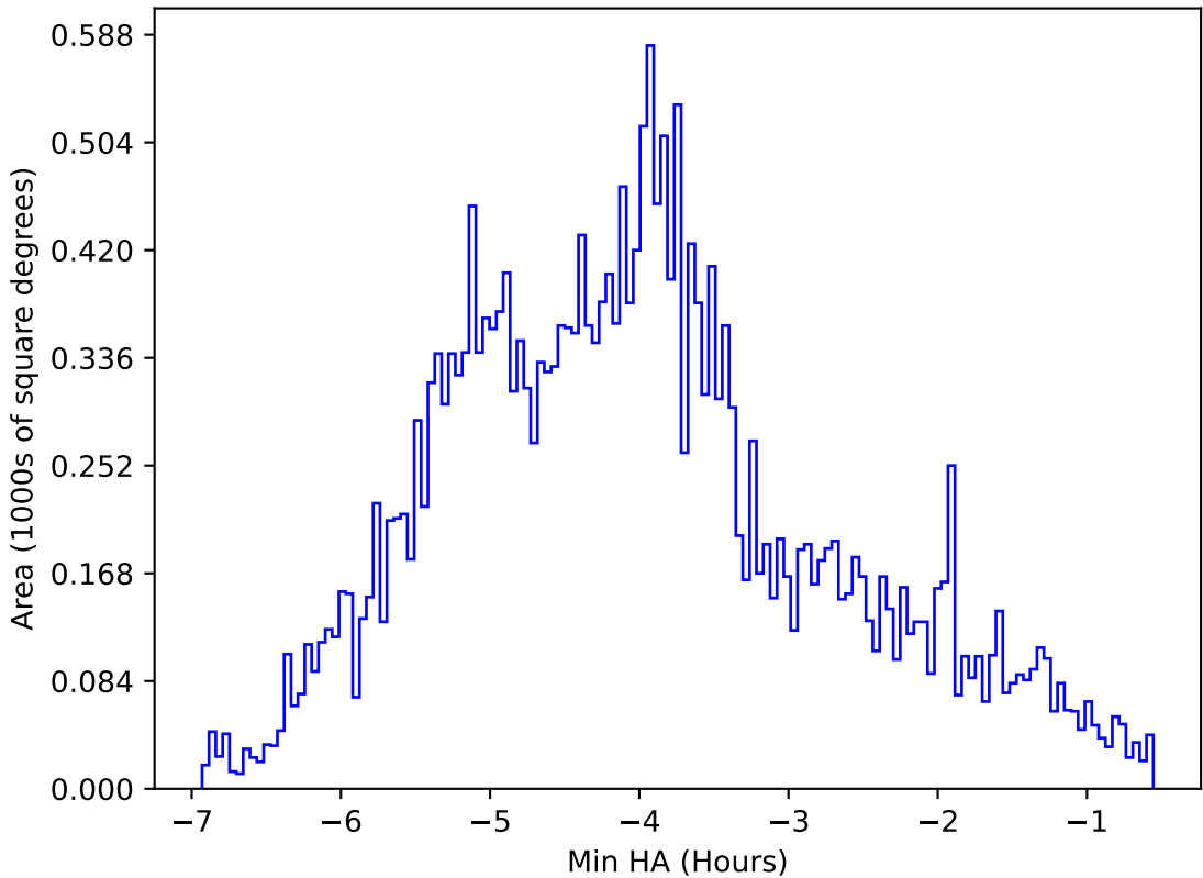
too_elab_heavy_r32_d2_gz_v3.4_10yrs All sky z band: Min HA
