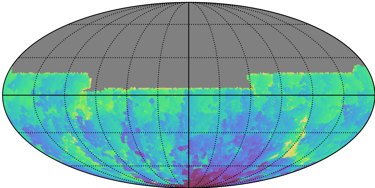
too_elab_heavy_r32_d2_gz_v3.4_10yrs All sky u band: Min HA
