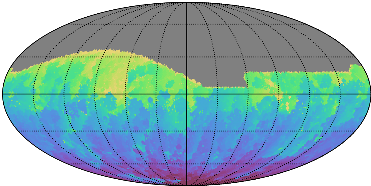
too_elab_heavy_r32_d2_gz_v3.4_10yrs All sky g band: Min HA
