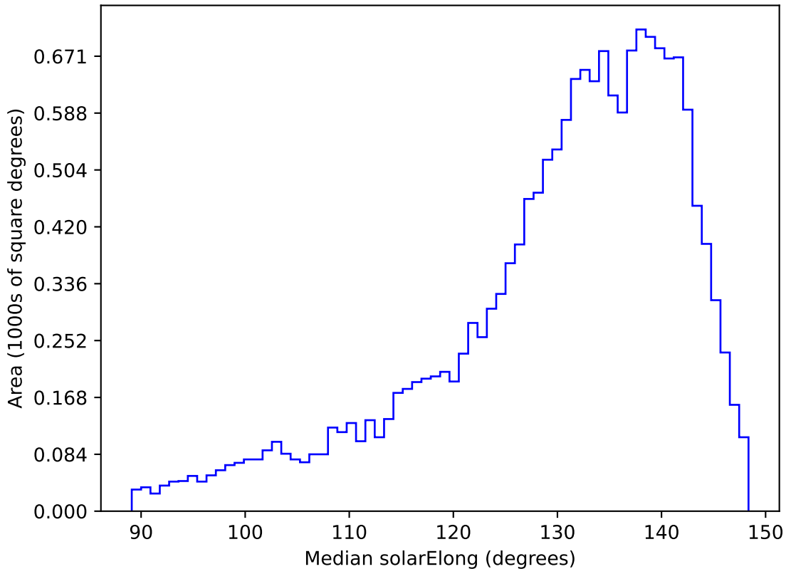
too_elab_heavy_r32_d2_gz_v3.4_10yrs WFD y band: Median solarElong
