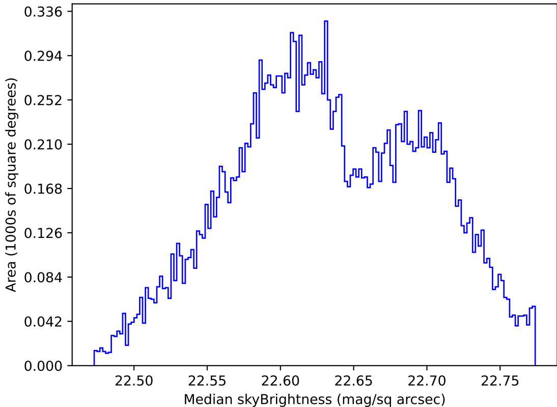
too_elab_heavy_r32_d2_gz_v3.4_10yrs Yr 1 u band: Median skyBrightness
