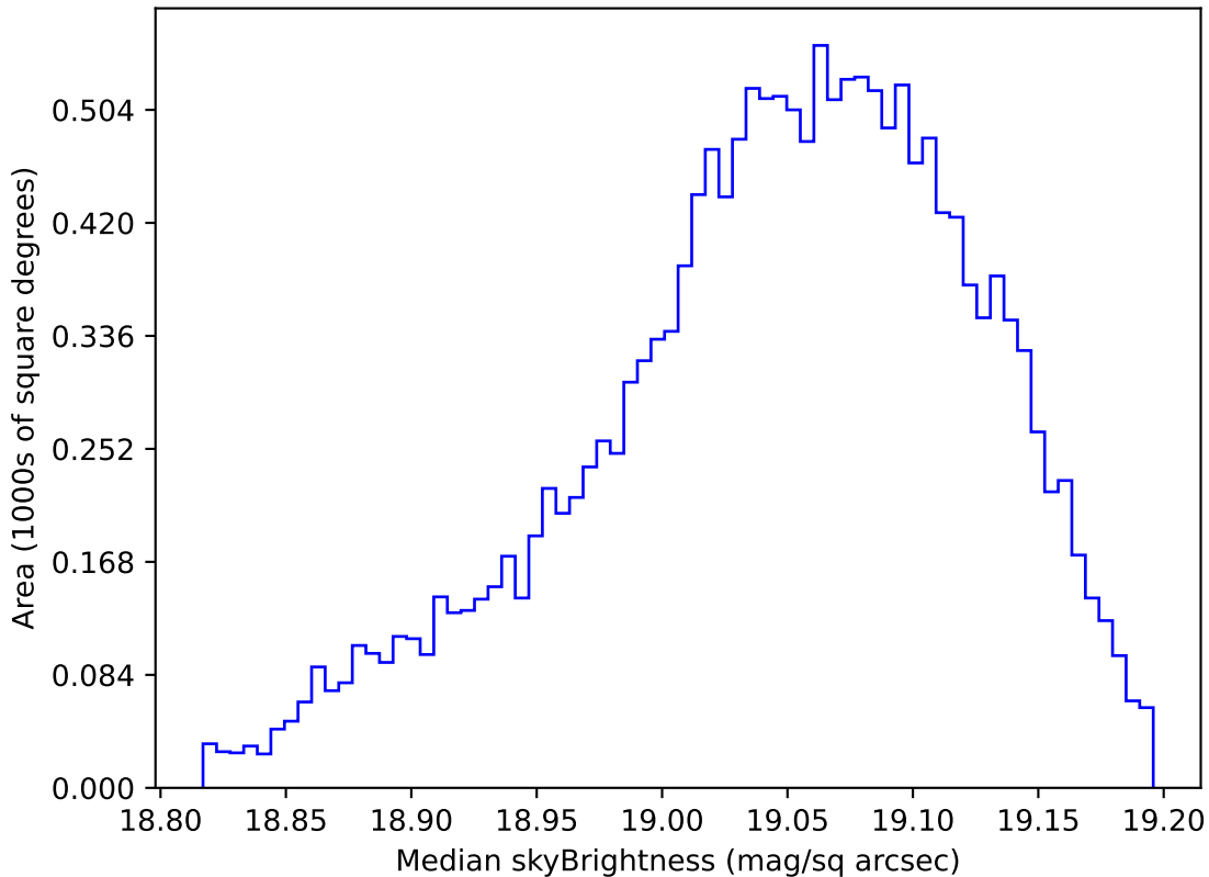
too_elab_heavy_r32_d2_gz_v3.4_10yrs WFD z band: Median skyBrightness
