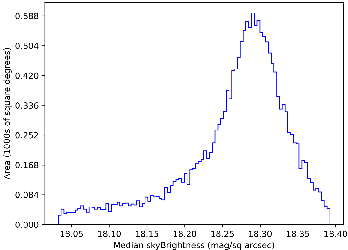
too_elab_heavy_r32_d2_gz_v3.4_10yrs WFD y band: Median skyBrightness
