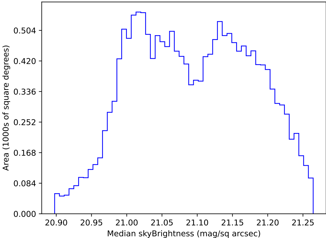
too_elab_heavy_r32_d2_gz_v3.4_10yrs WFD r band: Median skyBrightness
