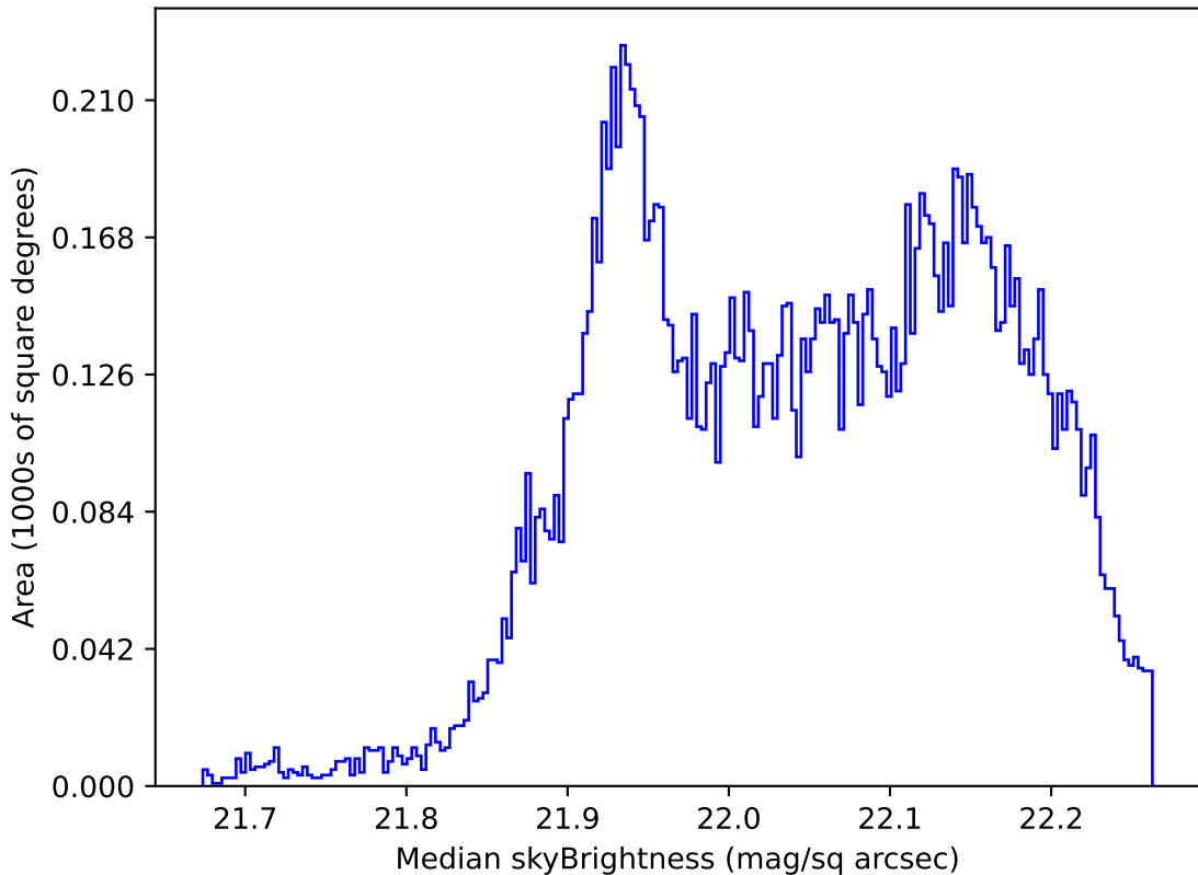
too_elab_heavy_r32_d2_gz_v3.4_10yrs WFD g band: Median skyBrightness
