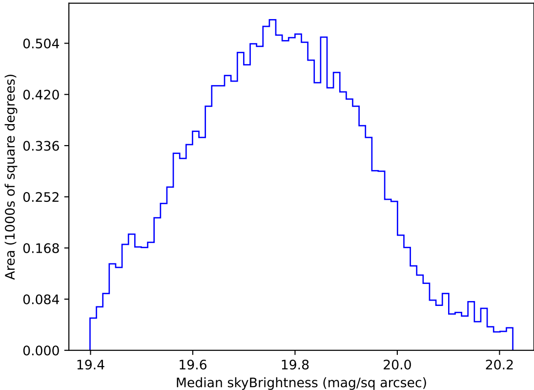
too_elab_heavy_r32_d2_gz_v3.4_10yrs WFD all bands: Median skyBrightness
