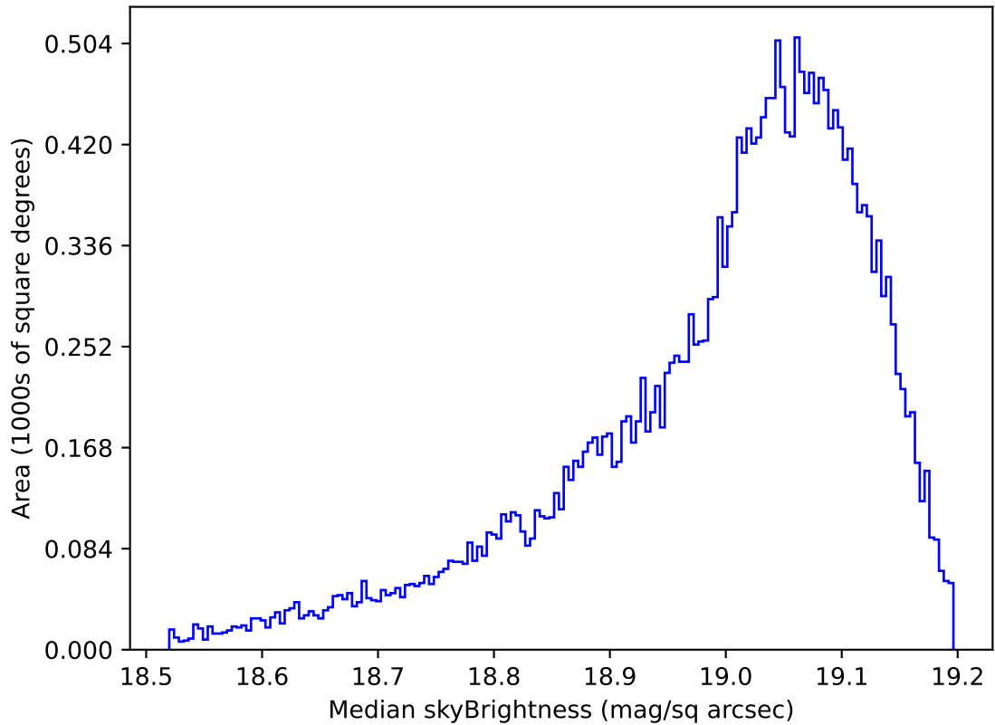
too_elab_heavy_r32_d2_gz_v3.4_10yrs All sky z band: Median skyBrightness
