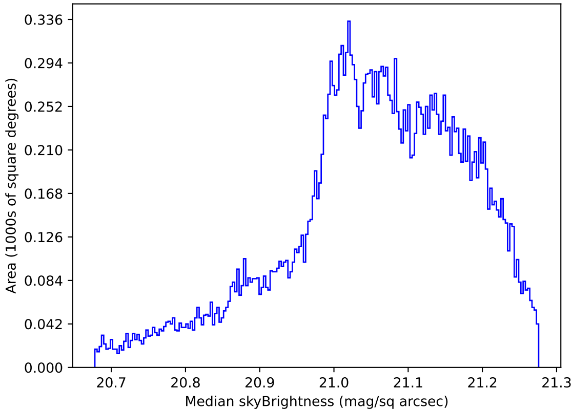
too_elab_heavy_r32_d2_gz_v3.4_10yrs All sky r band: Median skyBrightness
