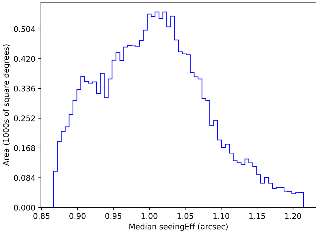
too_elab_heavy_r32_d2_gz_v3.4_10yrs WFD z band: Median seeingEff
