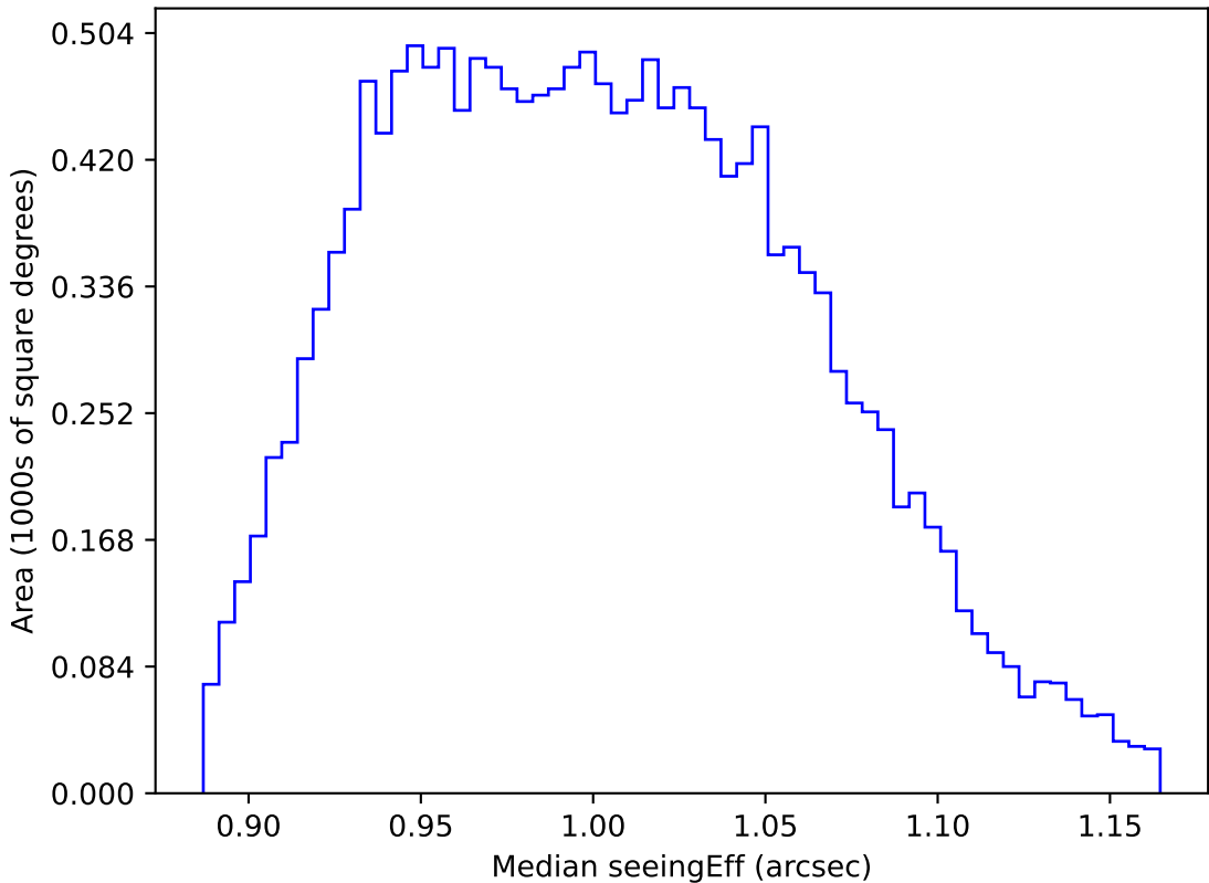
too_elab_heavy_r32_d2_gz_v3.4_10yrs WFD y band: Median seeingEff
