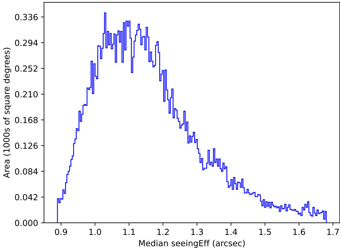
too_elab_heavy_r32_d2_gz_v3.4_10yrs All sky g band: Median seeingEff
