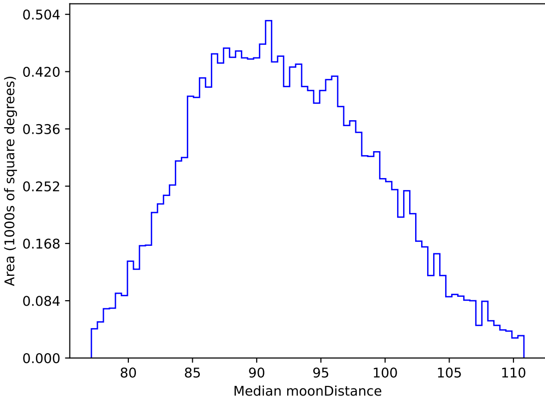
too_elab_heavy_r32_d2_gz_v3.4_10yrs WFD i band: Median moonDistance
