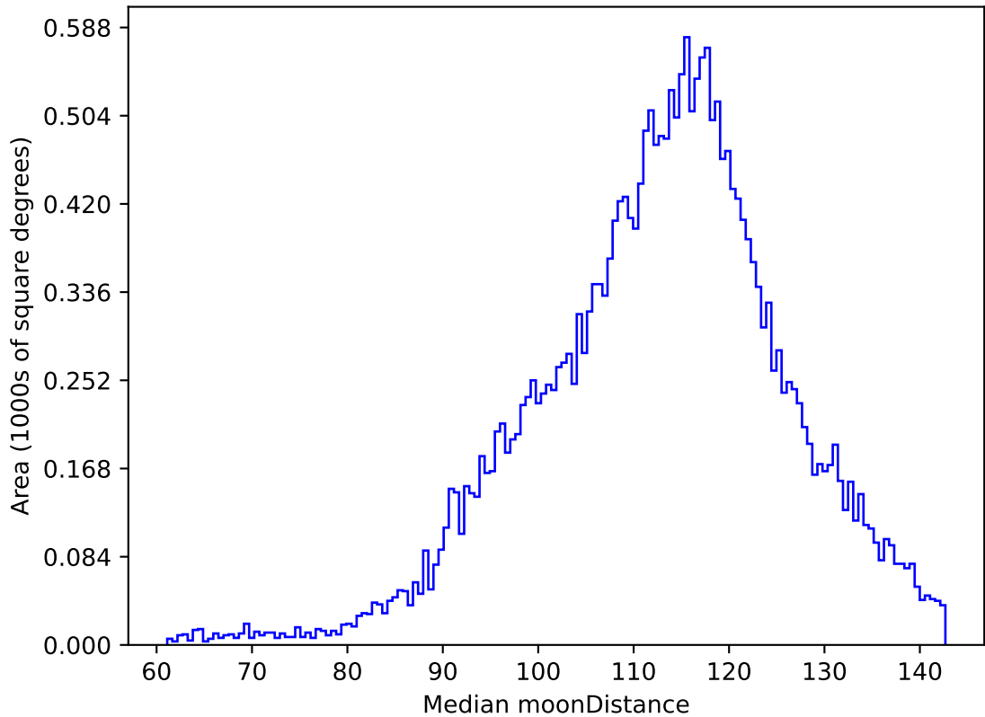
too_elab_heavy_r32_d2_gz_v3.4_10yrs All sky g band: Median moonDistance
