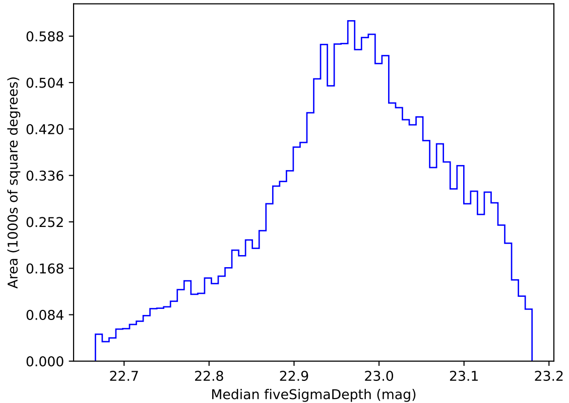
too_elab_heavy_r32_d2_gz_v3.4_10yrs WFD z band: Median fiveSigmaDepth
