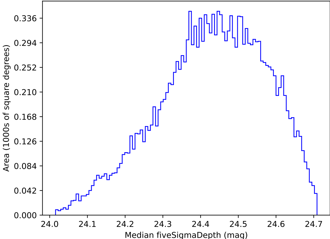
too_elab_heavy_r32_d2_gz_v3.4_10yrs WFD g band: Median fiveSigmaDepth
