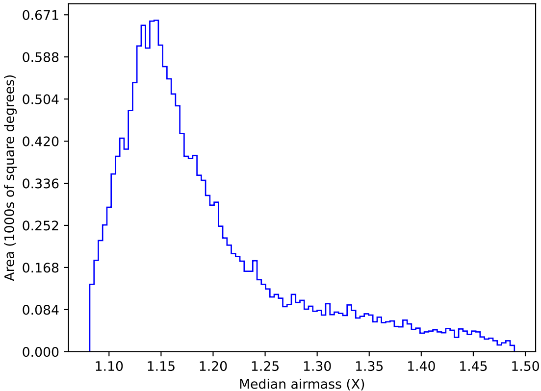
too_elab_heavy_r32_d2_gz_v3.4_10yrs WFD g band: Median airmass
