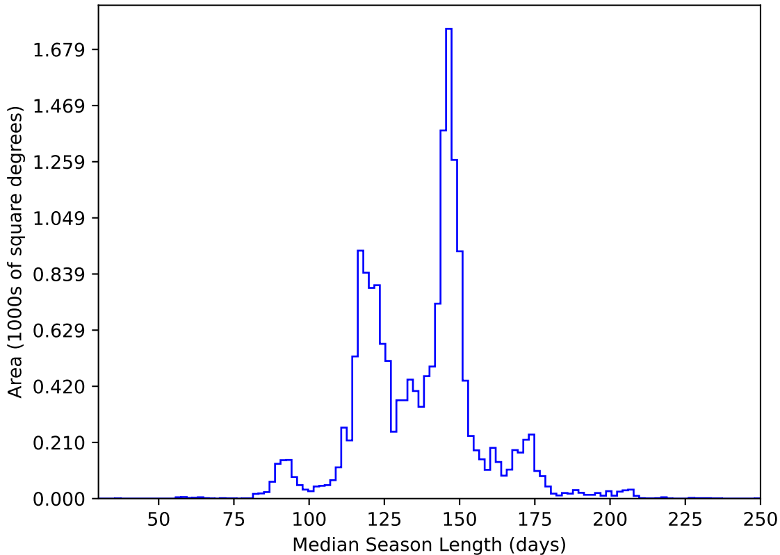
too_elab_heavy_r32_d2_gz_v3.4_10yrs WFD y band: Median Season Length
