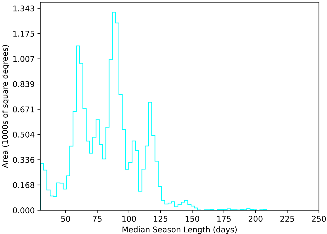
too_elab_heavy_r32_d2_gz_v3.4_10yrs WFD u band: Median Season Length
