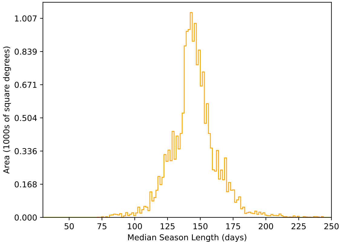
too_elab_heavy_r32_d2_gz_v3.4_10yrs WFD r band: Median Season Length
