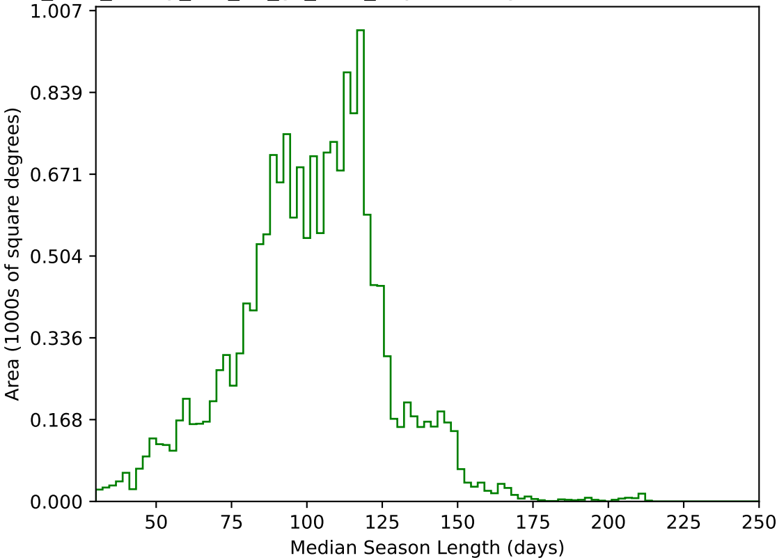
too_elab_heavy_r32_d2_gz_v3.4_10yrs WFD g band: Median Season Length
