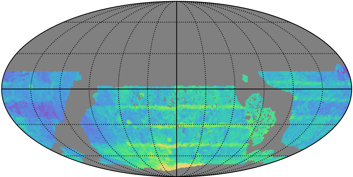
too_elab_heavy_r32_d2_gz_v3.4_10yrs WFD all bands: Median Season Length
