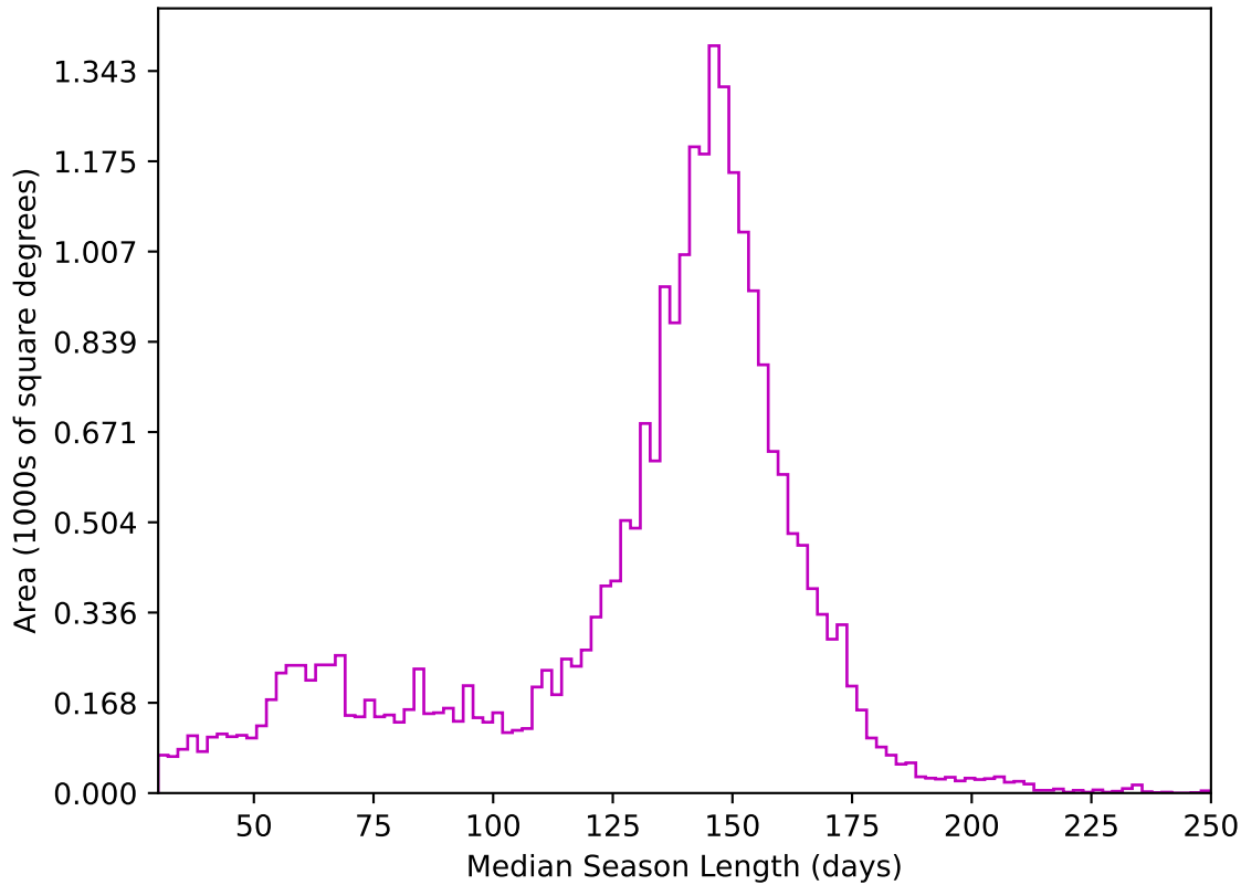
too_elab_heavy_r32_d2_gz_v3.4_10yrs All sky z band: Median Season Length
