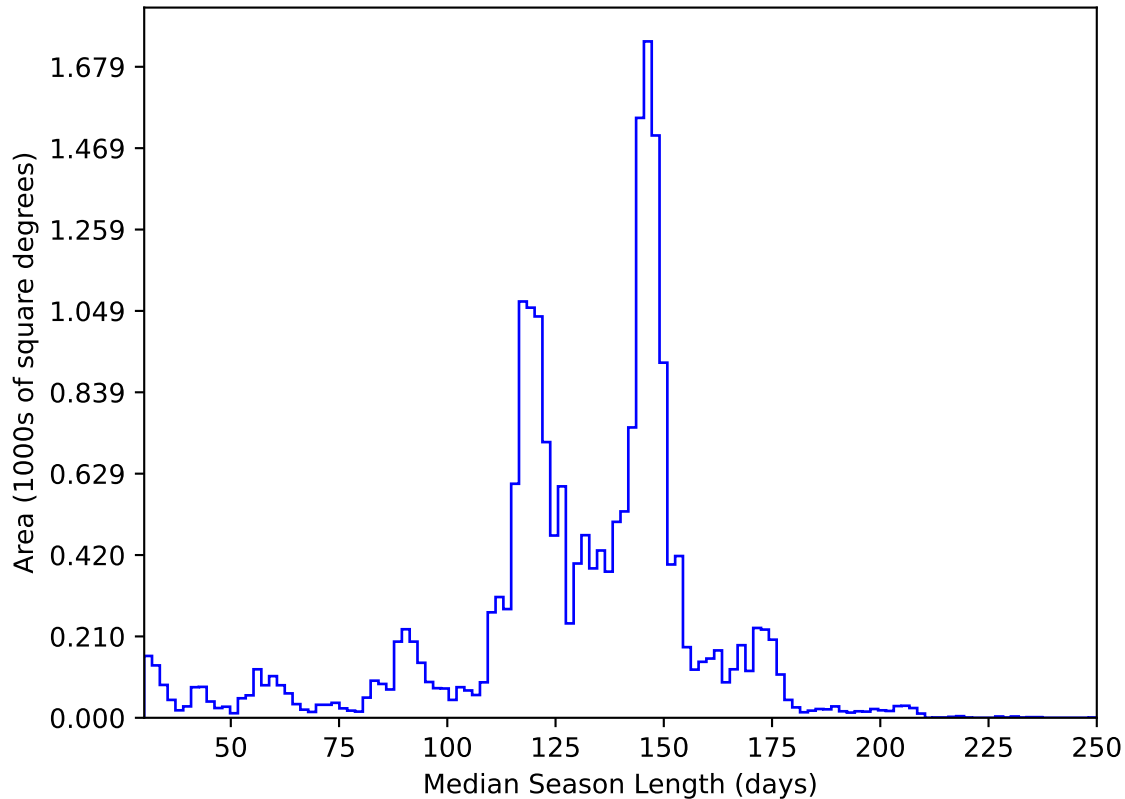
too_elab_heavy_r32_d2_gz_v3.4_10yrs All sky y band: Median Season Length
