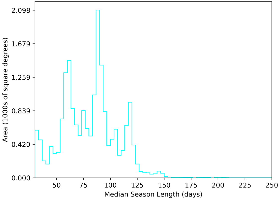
too_elab_heavy_r32_d2_gz_v3.4_10yrs All sky u band: Median Season Length
