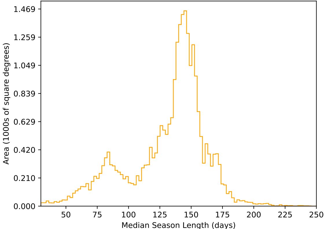
too_elab_heavy_r32_d2_gz_v3.4_10yrs All sky r band: Median Season Length
