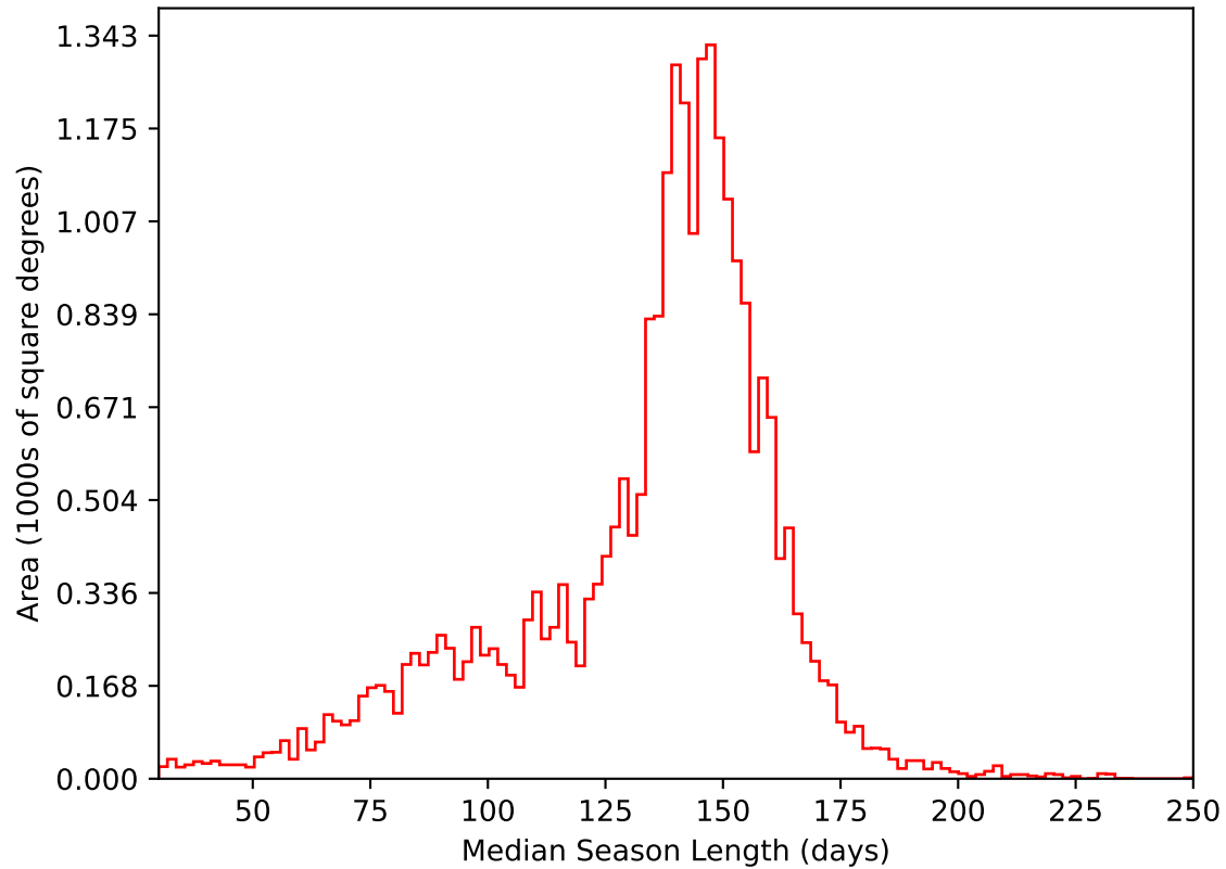
too_elab_heavy_r32_d2_gz_v3.4_10yrs All sky i band: Median Season Length
