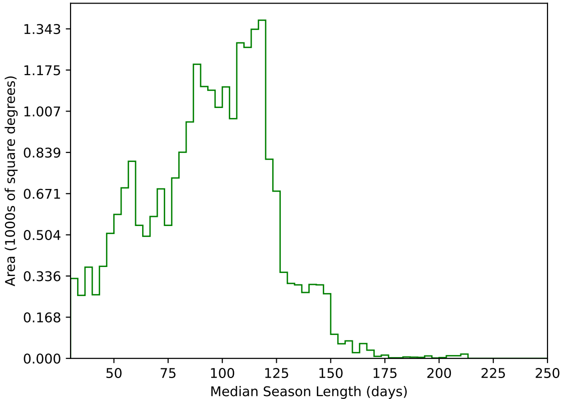
too_elab_heavy_r32_d2_gz_v3.4_10yrs All sky g band: Median Season Length
